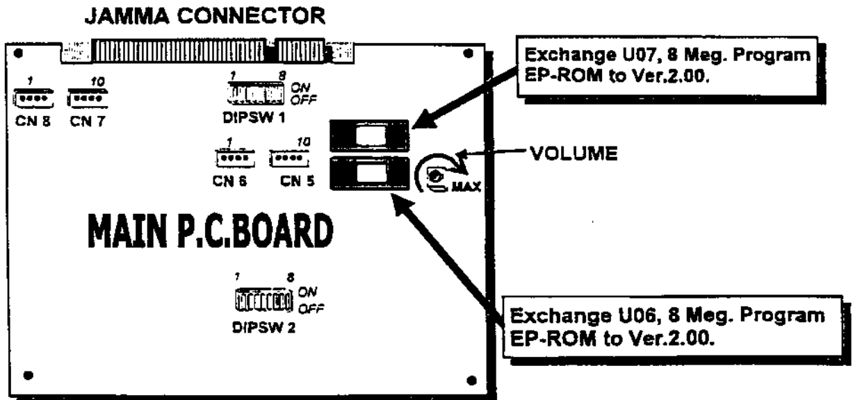
WING SHOOTING CHAMPIONSHIP, MAIN P.C.B. LAYOUT
